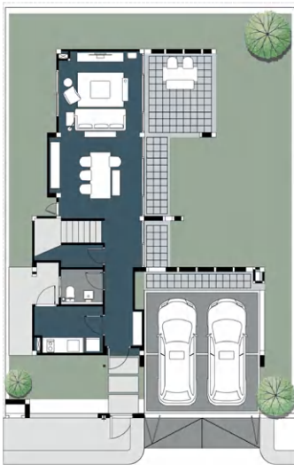
1 st FL.
